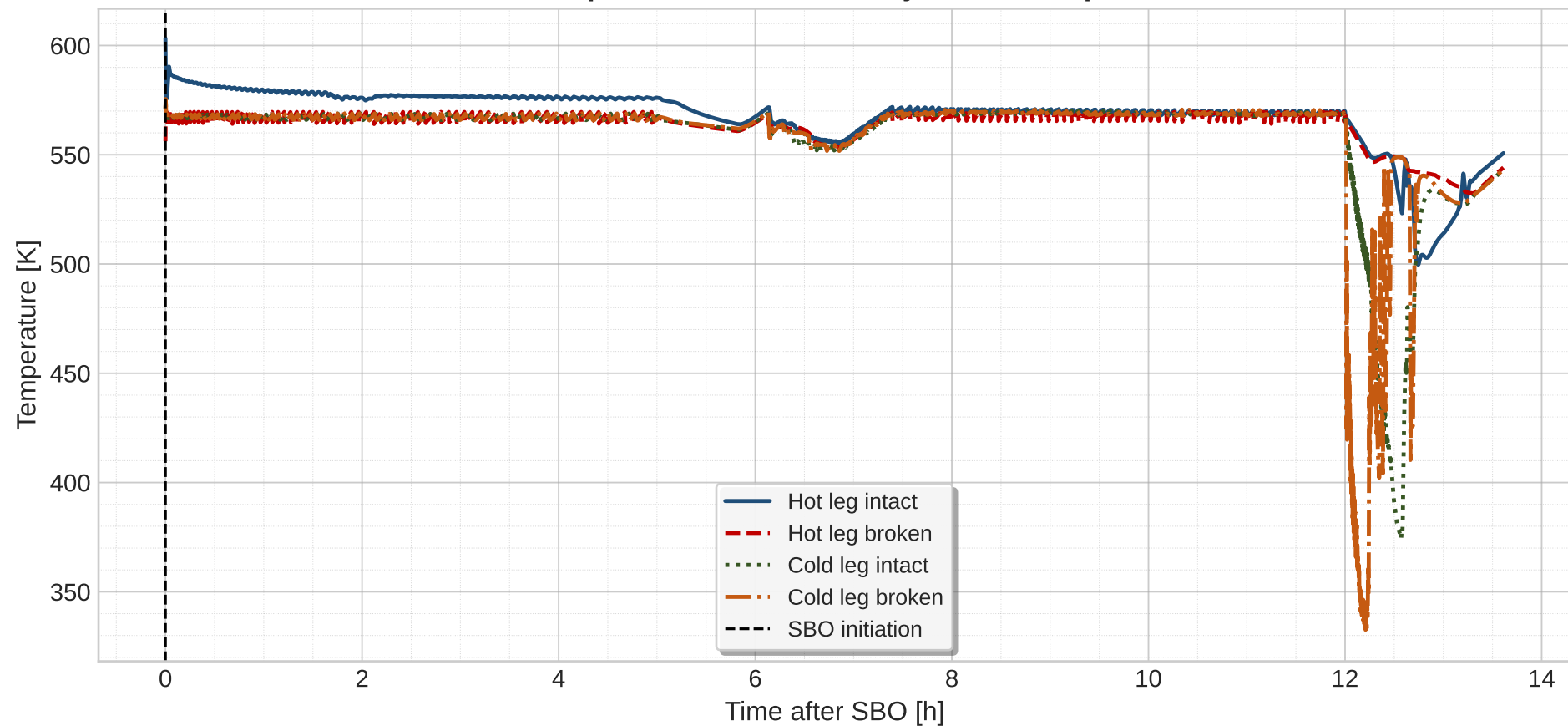
No SG Depressurization - Primary Circuit Temperatures
